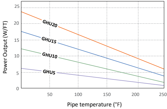
GHU Power-Temperature Characteristics
